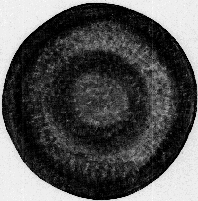
Fig. 4. Drawing of thin section of spherule of type 3. Magnified about 120 times.
