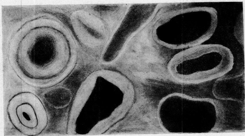
Fig. 1. Drawing of etched polished surface of oolite. Magnified about 50 times.
