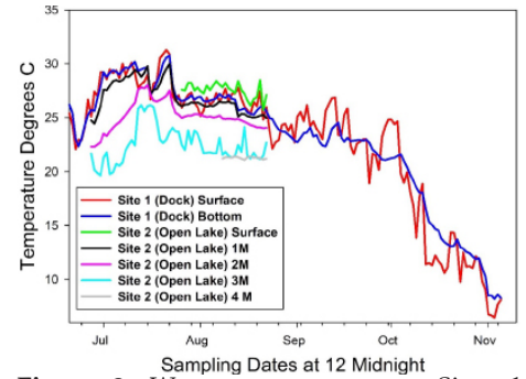
Figure 2. Water temperature at Sites 1 (Dock) and 2 (Open Lake).
